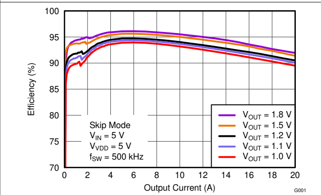
Figure 6-33. Efficiency vs Output Current
