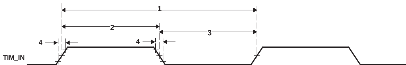
Figure 6-74. Timer Timing
