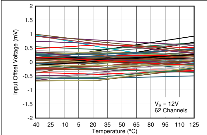
Figure 7-9. Input Offset Voltage vs. Temperature at 12V
