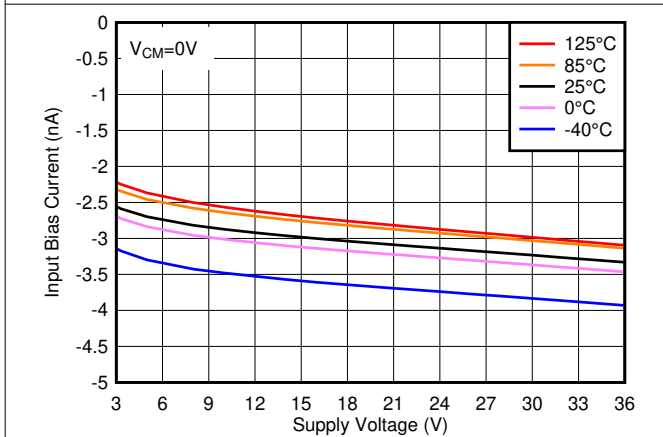
Figure 7-15. Input Bias Current vs. Supply Voltage
