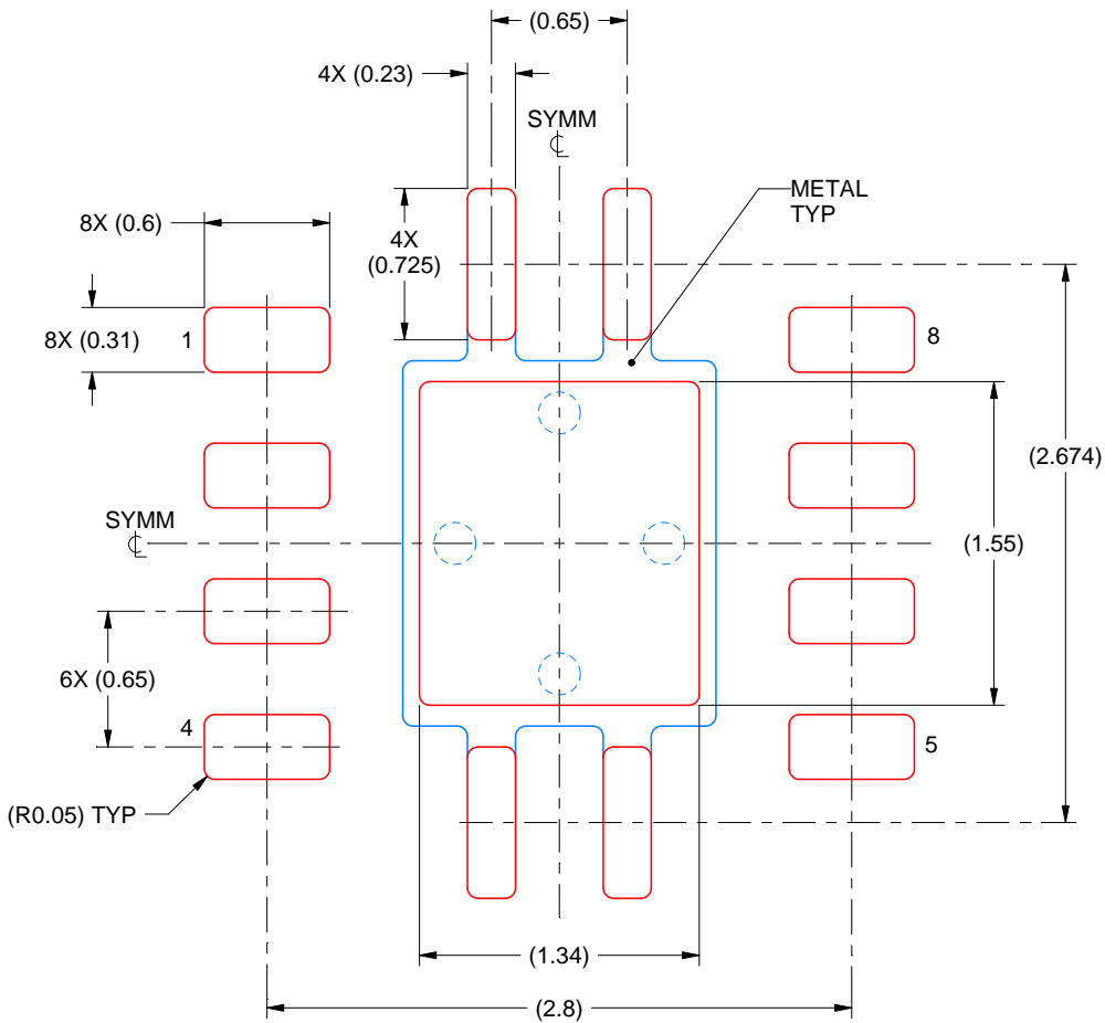
SOLDER PASTE EXAMPLE BASED ON 0.125 mm THICK STENCIL EXPOSED PAD 84% PRINTED SOLDER COVERAGE BY AREA SCALE:25X
