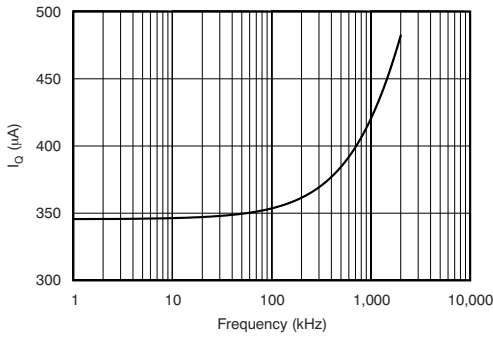
Figure 7-17. Active I_Q vs. I^2C Clock Frequency
