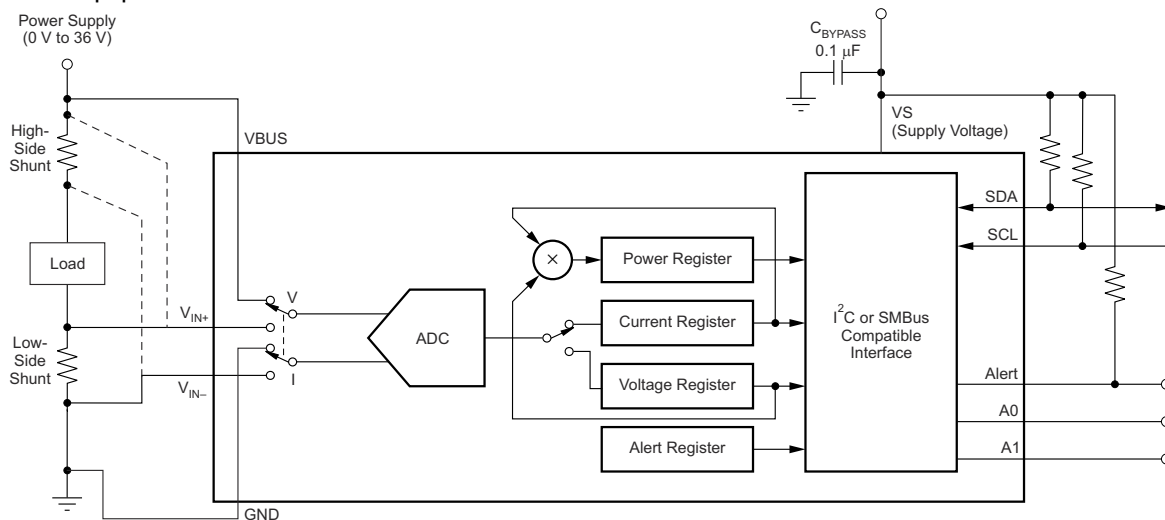
Typical Application
