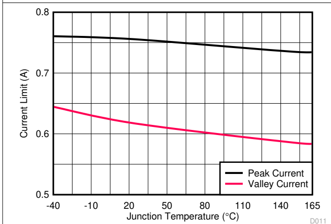
Figure 6-9. Peak and Valley Current Limit versus Temperature
