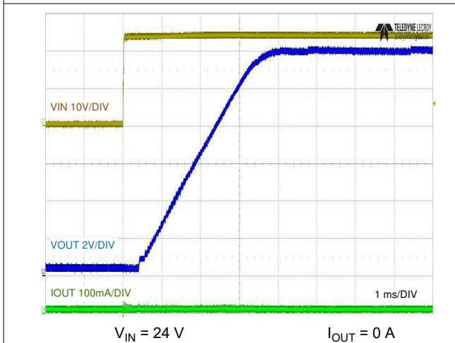
Figure 8-6. No-Load Start-up with VIN
