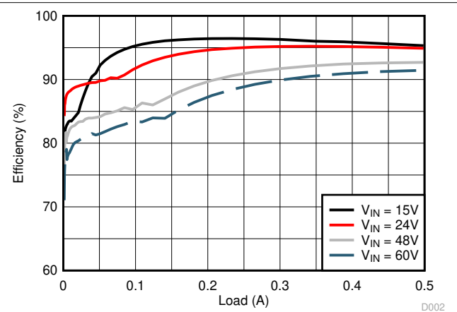
Figure 8-3. Conversion Efficiency (Linear Scale)
