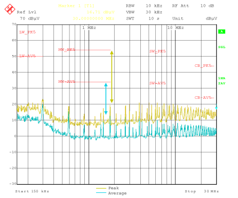
Figure 8-14. No-Load Switching
