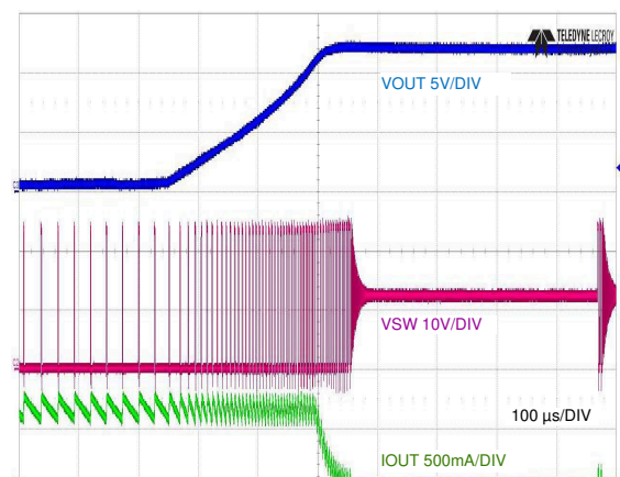
Figure 8-10. Pre-bias Start-up with EN/UVLO
