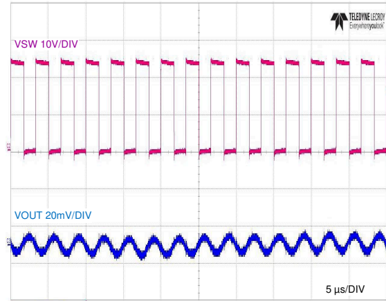
Figure 8-15. Full-Load Switching
