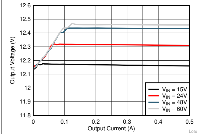
Figure 8-4. Load and Line Regulation Performance
