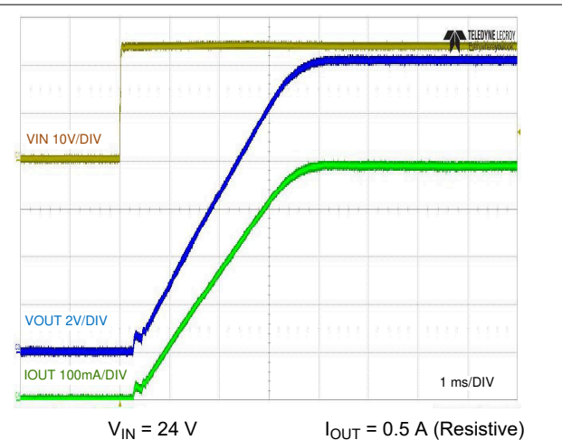
Figure 8-7. Full-Load Start-up with VIN
