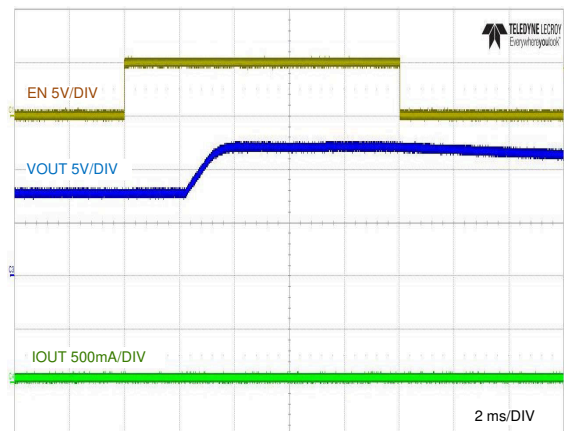
Figure 8-8. No-Load Start-up and Shutdown with EN/UVLO
