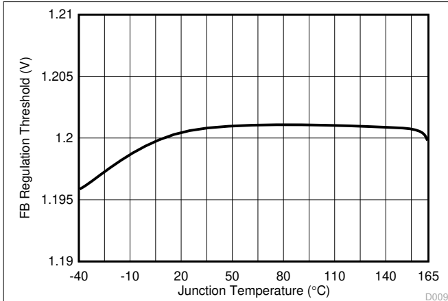
Figure 6-7. Feedback Comparator Threshold versus Temperature
