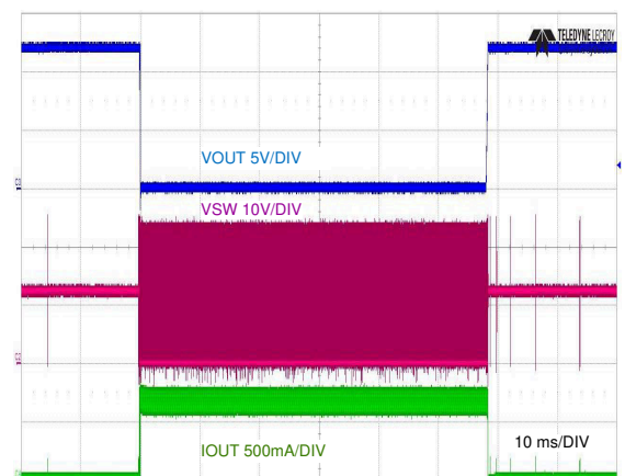
Figure 8-11. Short Circuit Applied
