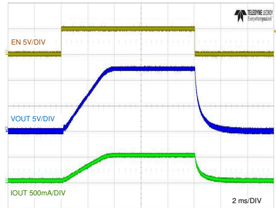
Figure 8-9. Full-Load Start-up and Shutdown with EN/UVLO
