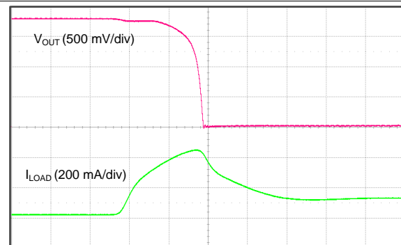
Time (100 \mu\text{s}/\text{div} ) TLV73318PDBV, 1\text{-}\mu\text{F} output capacitor
