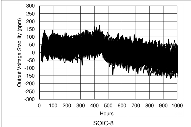
Figure 7-27. REF50xx Long-Term Stability (First 1000 Hours)
