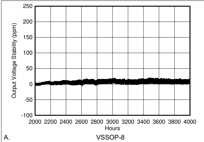
A. Figure 7-25. REF50xx Long-Term Stability (Second 2000 Hours)
