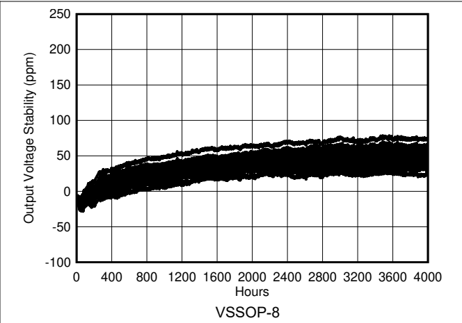
Figure 7-26. REF50xx Long-Term Stability (4000 Hours)
