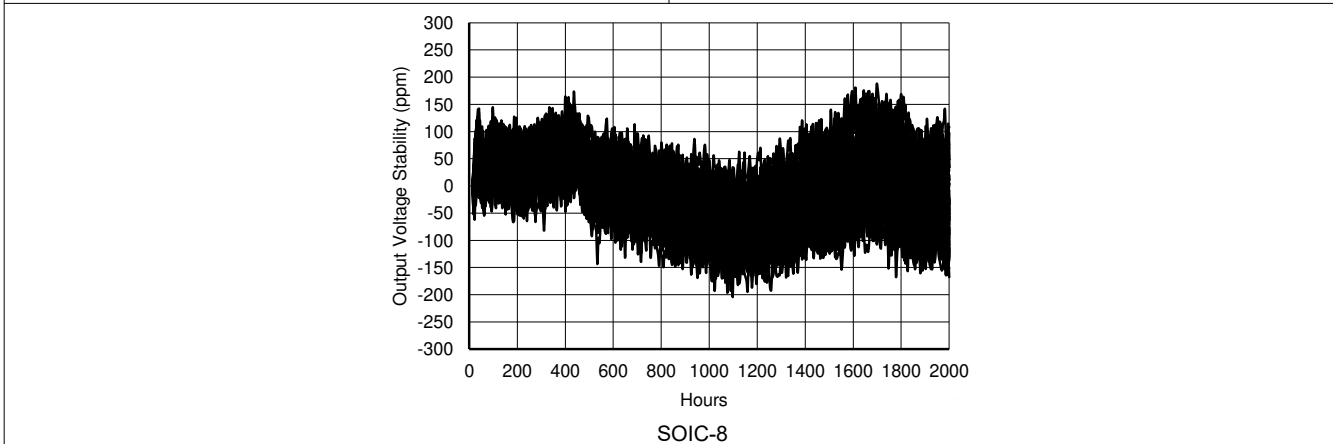
Figure 7-29. REF50xx Long-Term Stability (2000 Hours)
