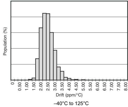
Figure 7-2. Temperature Drift
