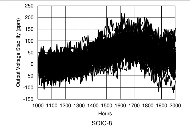
Figure 7-28. REF50xx Long-Term Stability (Second 1000 Hours)
