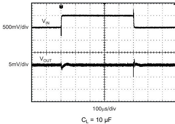
Figure 7-21. Line Transient
