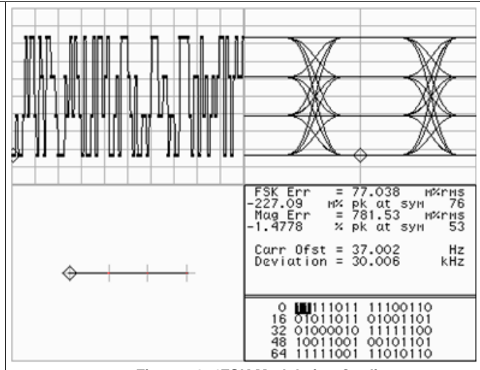
Figure 71. 4FSK Modulation Quality
