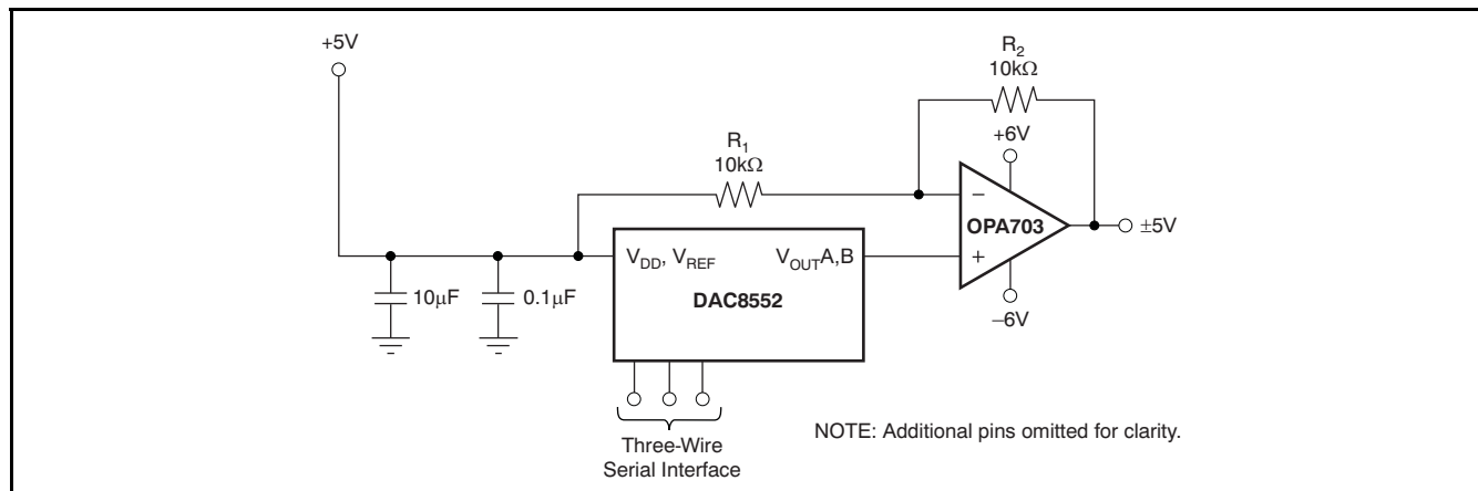
Figure 51. Bipolar Operation with the DAC8552
