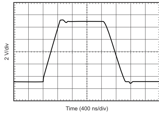
图 6-30. Large-Signal Step Response
