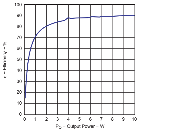
Gain = 20 dB V_{CC} = 12\text{ V} Z_L = 4\ \Omega + 33\ \mu\text{H}
