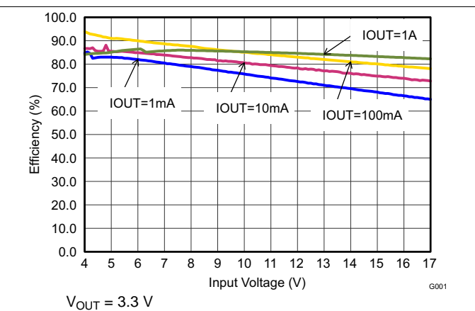
Figure 11. Efficiency vs Input Voltage
