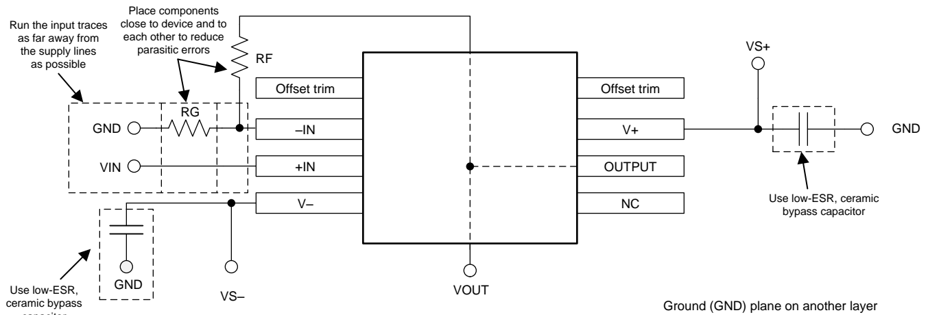
Figure 32. OPA134 Layout Example for the Noninverting Configuration
