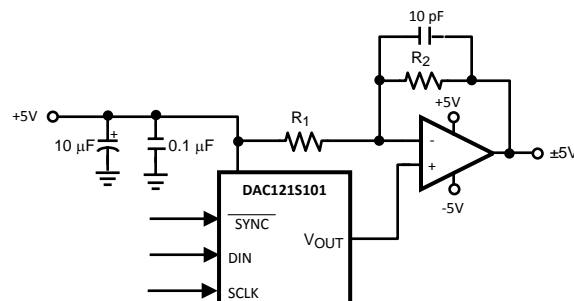
Figure 39. Bipolar Operation
