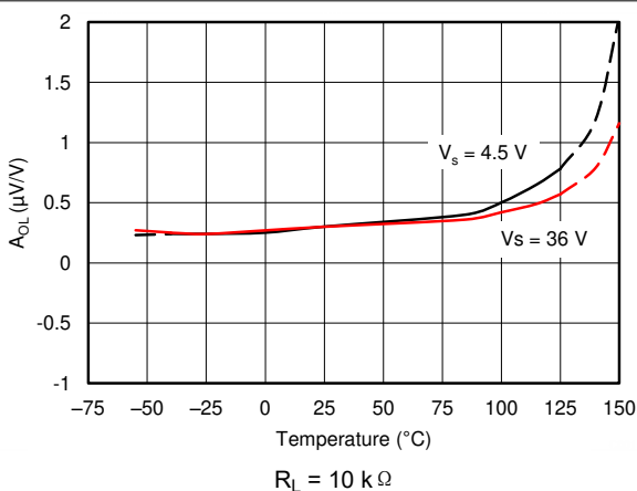
图 7-23. Open-Loop Gain vs Temperature
