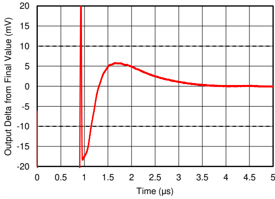
G = 1 , C_L = 10\text{ pF} , 0.1% settling = \pm 10\text{ mV}
