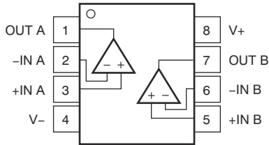
图 6-1. D (SOIC-8) Package, Top View
