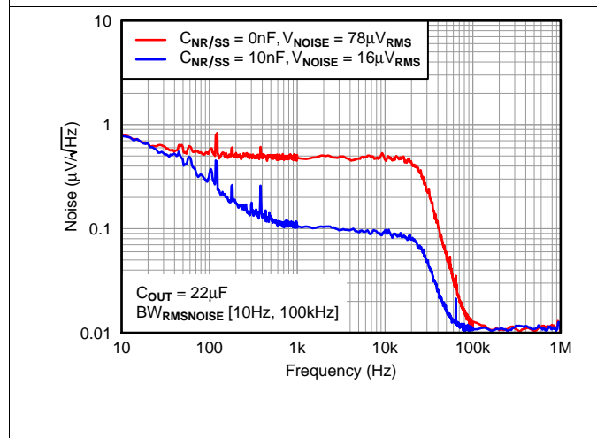
Figure 21. Output Spectral Noise Density vs C_{NR/SS}
