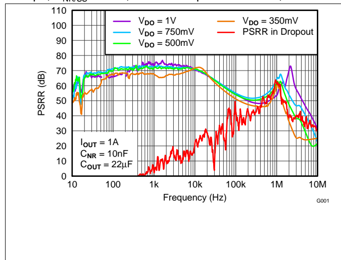
Figure 19. Power-Supply Rejection Ratio vs V_{DO}
