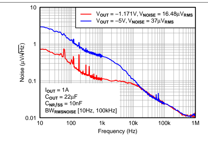
Figure 22. Output Spectral Noise Density vs V_{OUT(nom)}
