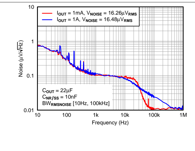
Figure 20. Output Spectral Noise Density vs Output Current
