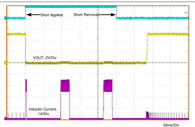
Figure 7-6. Short-Circuit Transient and Recovery
