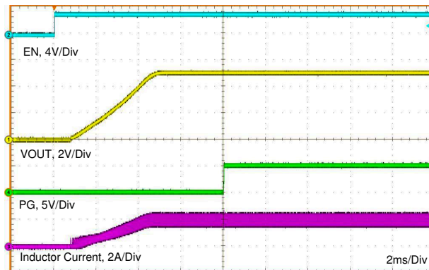
Figure 7-3. Precision Enable Behavior
