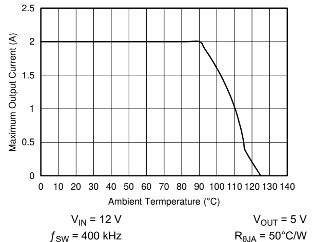
Figure 8-8. Maximum Output Current versus Ambient Temperature
