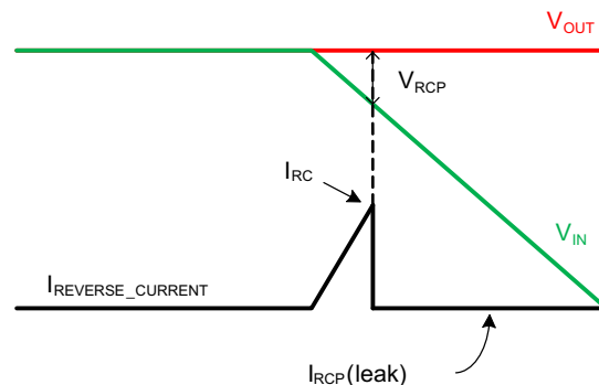
Figure 49. Reverse Current
