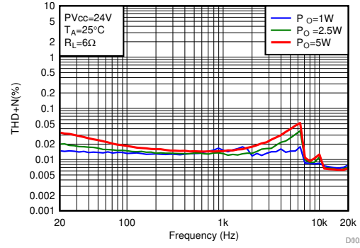
图 6-8. THD+N vs Frequency-BTL
