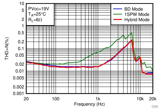
图 6-10. THD+N vs Frequency-BTL
