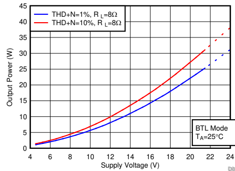
图 6-48. Output Power vs Supply Voltage
