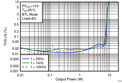
图 6-44. THD+N vs Output Power
