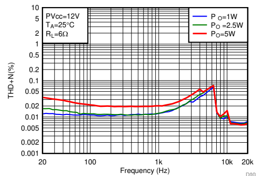
图 6-4. THD+N vs Frequency-BTL
