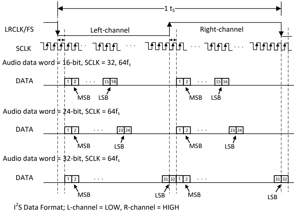
I²S Data Format; L-channel = LOW, R-channel = HIGH
