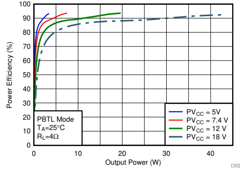
图 6-84. Efficiency vs Output Power
