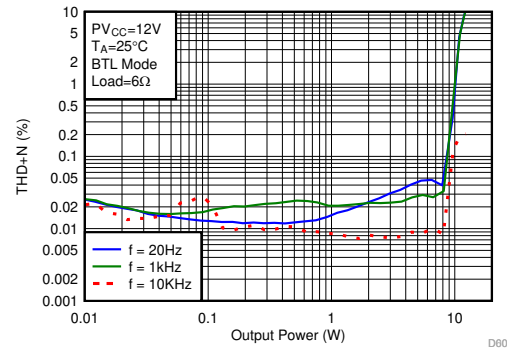
图 6-42. THD+N vs Output Power
