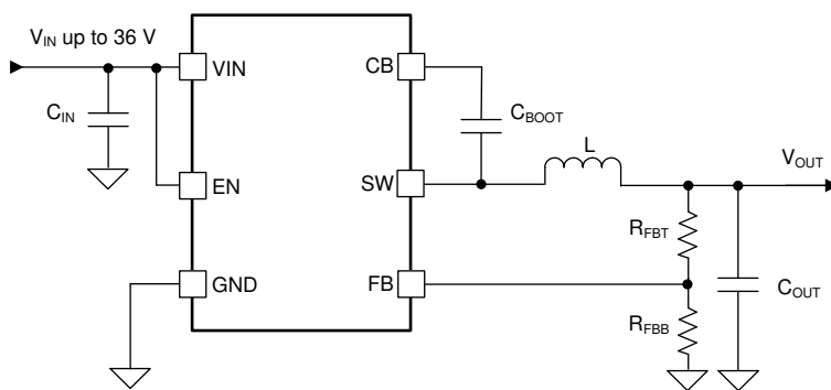
Simplified Schematic
