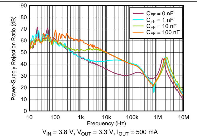
Figure 32. PSRR vs Frequency and C_{FF}
