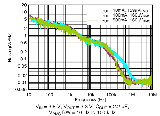
Figure 35. Output Spectral Noise Density
