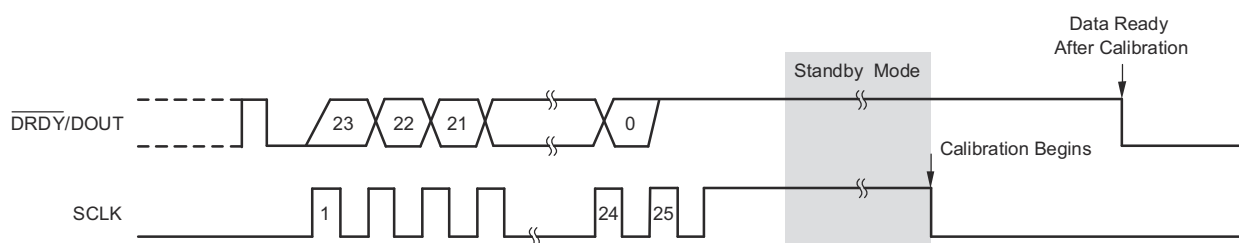
图 8-16. Summary of Serial Interface Waveforms
