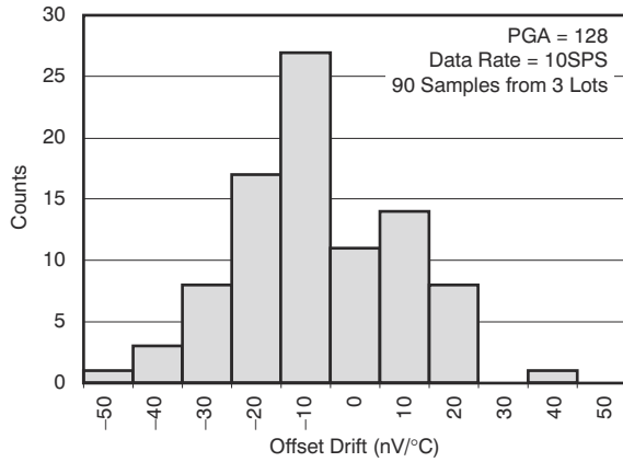
图 6-13. Offset Drift (-40°C to +25°C)
