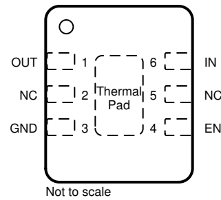
NC = no internal connection. 图 4-4. DRV Package, 6-Pin WSON With Exposed Thermal Pad (Top View)
