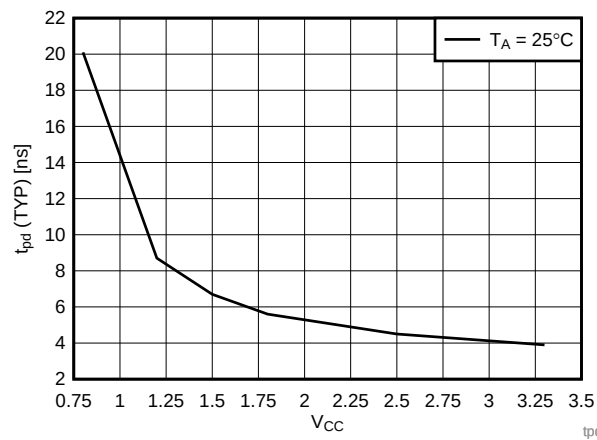
Figure 1. Typical Propagation Delay vs. Supply Voltage ( C_L = 15\text{ pF} )
