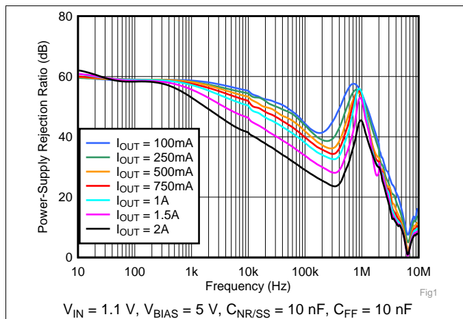
图 1. PSRR vs Frequency and I_{OUT}
