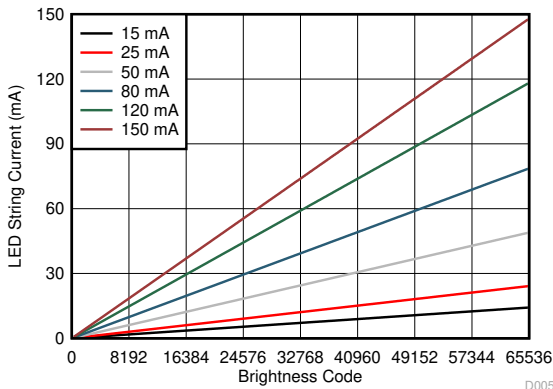
Figure 6-6. Current Linearity
