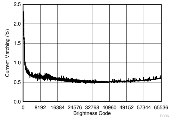
Figure 6-7. Current Matching
