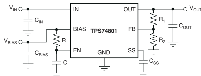
Figure 6-1. Soft-Start Delay Using an RC Circuit to Enable the Device
