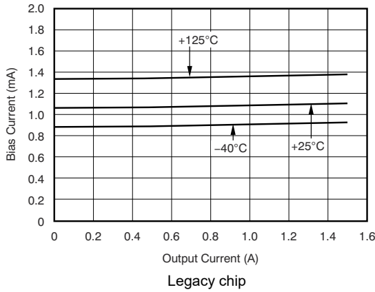
Figure 5-21. BIAS Pin Current vs Output Current and Temperature (T J )
