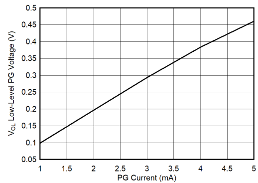
Figure 5-28. Low-Level PG Voltage vs Current
