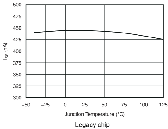
Figure 5-25. Soft-Start Charging Current ( I_{SS} ) vs Temperature ( T_J )
