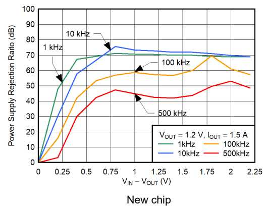
Figure 5-18. V IN PSRR vs (V IN - V OUT )
