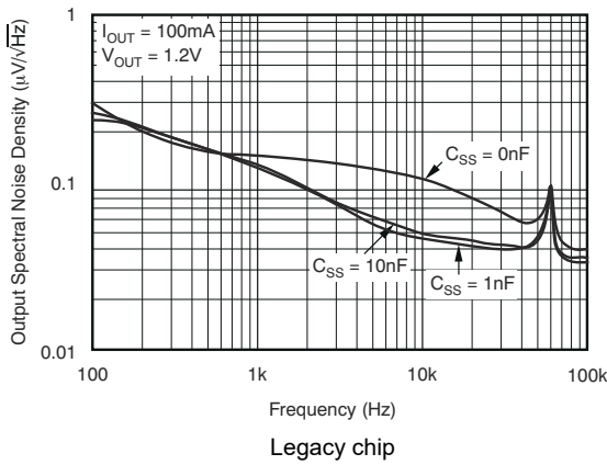
Figure 5-19. Noise Spectral Density
