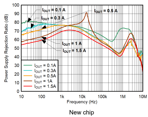
Figure 5-16. V IN PSRR vs Frequency
