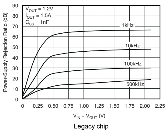
Figure 5-17. V IN PSRR vs (V IN - V OUT )
