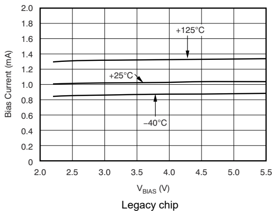
Figure 5-23. BIAS Pin Current vs V BIAS and Temperature (T J )
