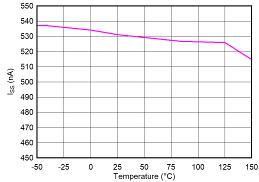
Figure 5-26. Soft-Start Charging Current ( I_{SS} ) vs Temperature ( T_J )
