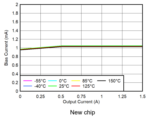
Figure 5-22. BIAS Pin Current vs Output Current and Temperature (T J )
