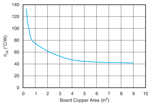
Figure 7-4. R_{\theta JA} vs Board Size
