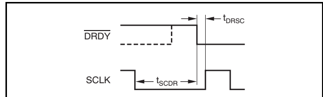
Figure 59. SCLK to \overline{DRDY} Timing
