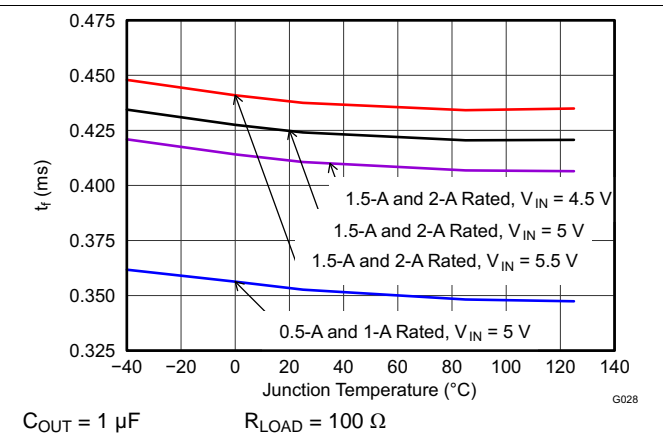
Figure 16. Output Fall Time ( T_F ) vs Temperature
