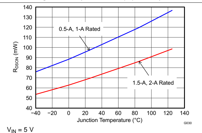
Figure 18. Input-Output Resistance ( R_{DS(ON)} ) vs Temperature
