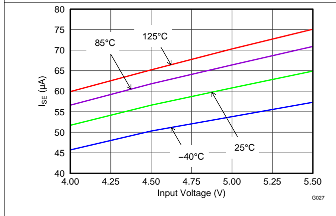
Figure 15. Enabled Supply Current ( I_{SE} ) vs Input Voltage
