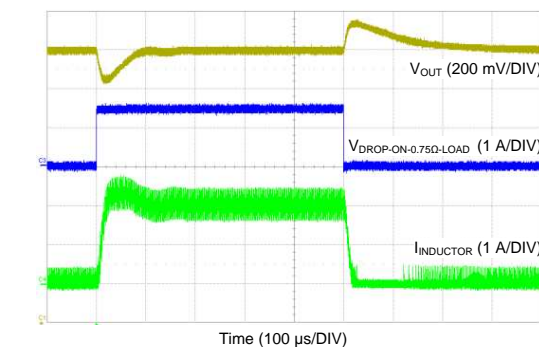
Figure 49. Output Voltage Regulation
