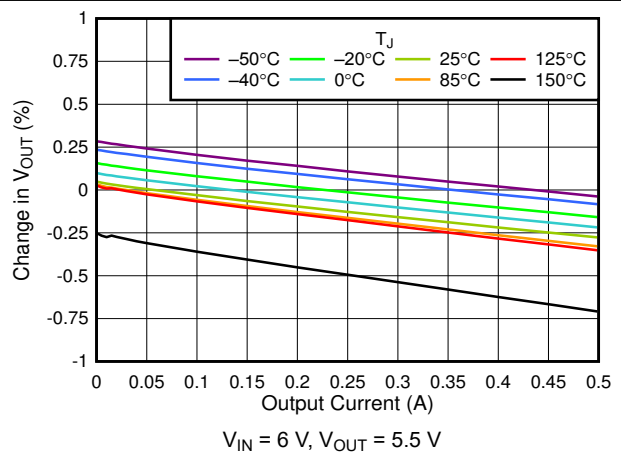
V_{IN} = 6\text{ V} , V_{OUT} = 5.5\text{ V} Figure 6-18. 5.5-V Load Regulation vs I_{OUT}
