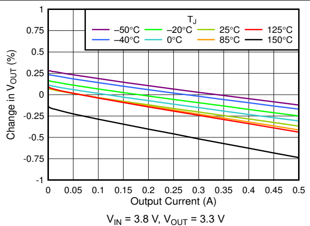
V_{IN} = 3.8\text{ V} , V_{OUT} = 3.3\text{ V} Figure 6-16. 3.3-V Load Regulation vs I_{OUT}
