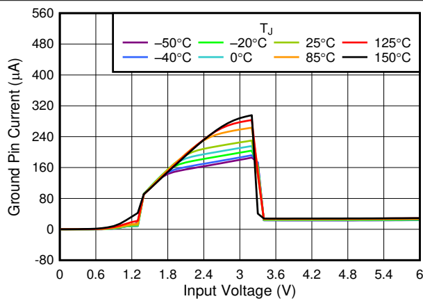
V_{OUT} = 3.3\text{ V} , I_{OUT} = 0\text{ mA} Figure 6-15. I_Q vs V_{IN}
