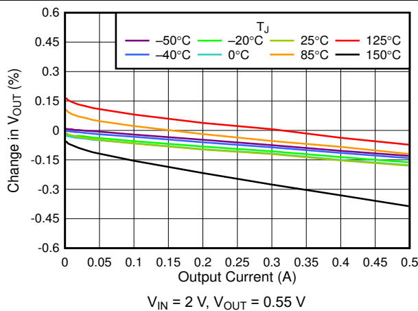
V_{IN} = 2\text{ V} , V_{OUT} = 0.55\text{ V} Figure 6-17. 0.55-V Load Regulation vs I_{OUT}
