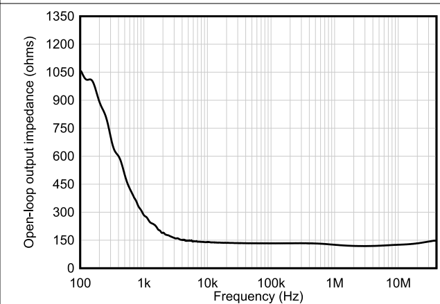
Figure 6-24. Open-Loop Output Impedance vs Frequency
