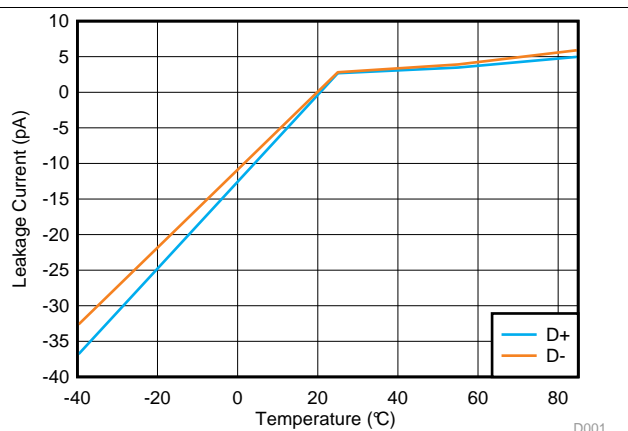
Figure 2. Leakage Current vs Temperature (V IO = 2.5 V)
