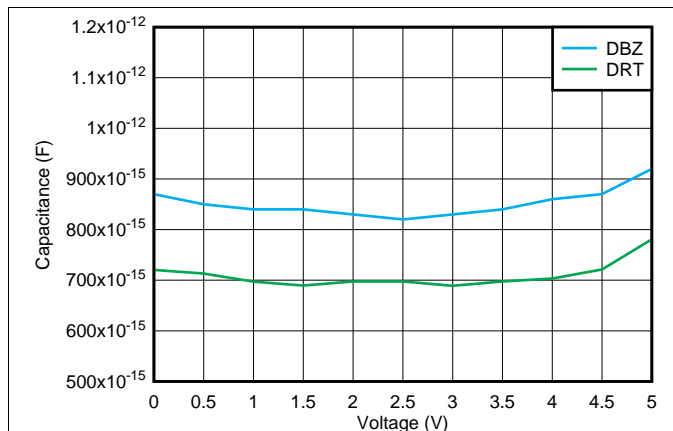
Figure 1. I/O Capacitance vs I/O Voltage (T A = 25°C)
