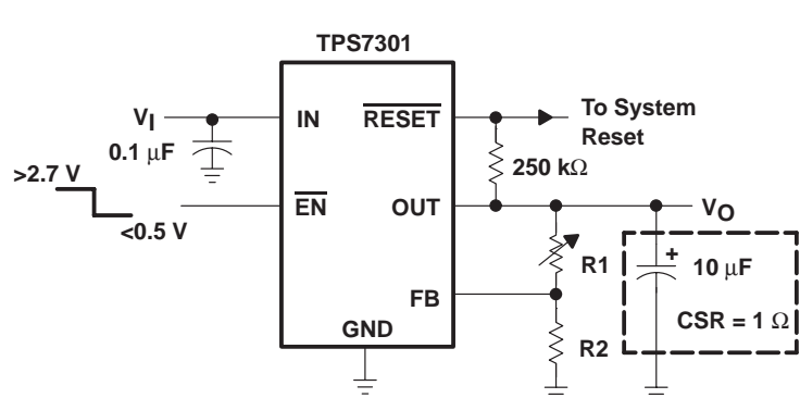
Figure 48. TPS7301 Adjustable LDO Regulator Programming
