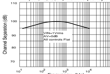
Fig.10 Input Separation (L1,L2,L3,L4) vs. Frequency
