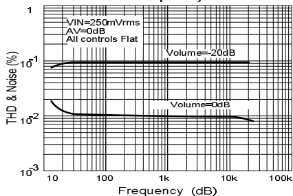
Fig.7 Distortion & Noise vs. Frequency
