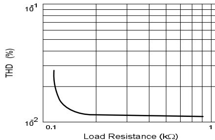
Fig.8 Distortion vs. Load Resistance
