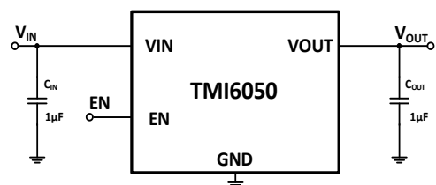
Figure 2. TMI6050 fixed output Circuit
