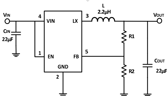
Figure 1. Basic Application Circuit
