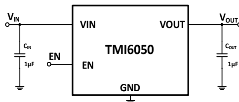
Figure 2. TMI6050 fixed output Circuit
