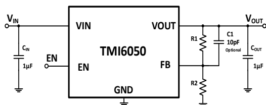
Figure 1. TMI6050 adjustable output Circuit
