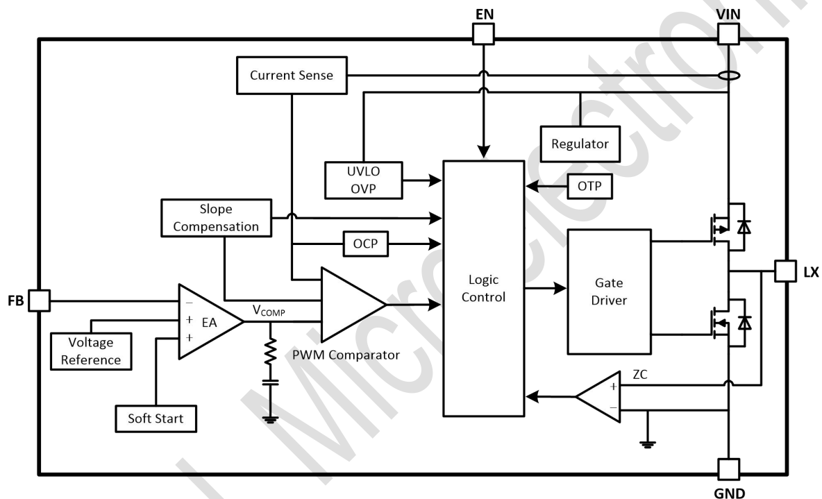
Figure 2. TMI3408C Block Diagram
