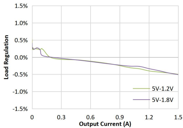
Load Regulation
