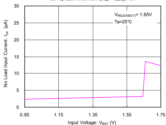
XC9140x18x(V OUT =1.8V)
