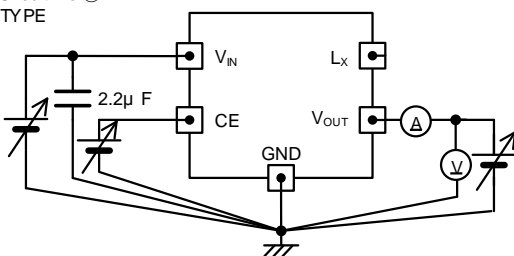
< Circuit No.⑦ > B TYPE
