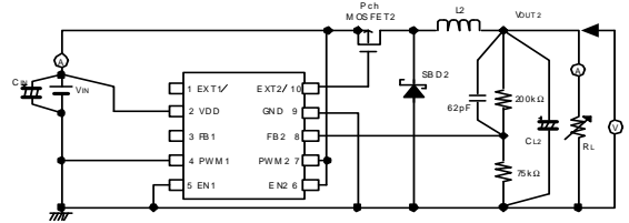
Circuit
