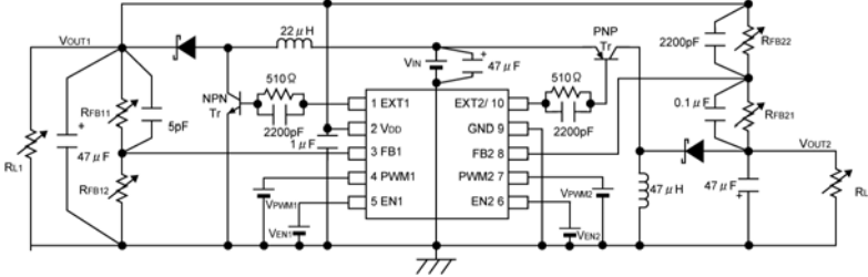
Circuit 2
