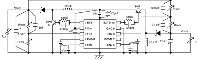
Circuit 1
