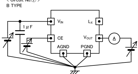
< Circuit No.⑦ >
