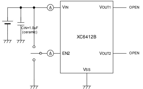
Circuit ②
