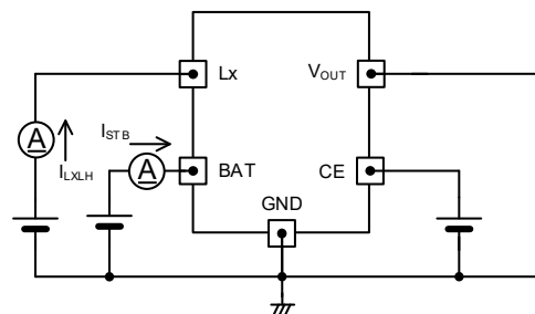
< Circuit No.⑧ >
