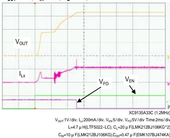
(30) Soft-start
