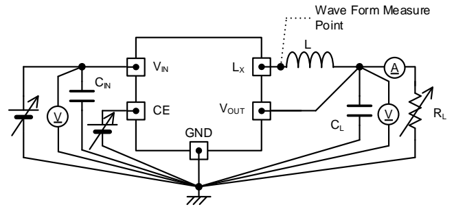
< Circuit No.② >
