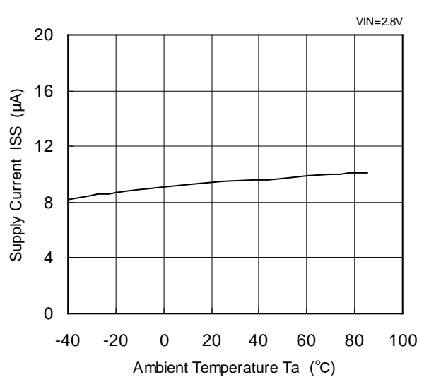
XC6202P182(1.8V)
