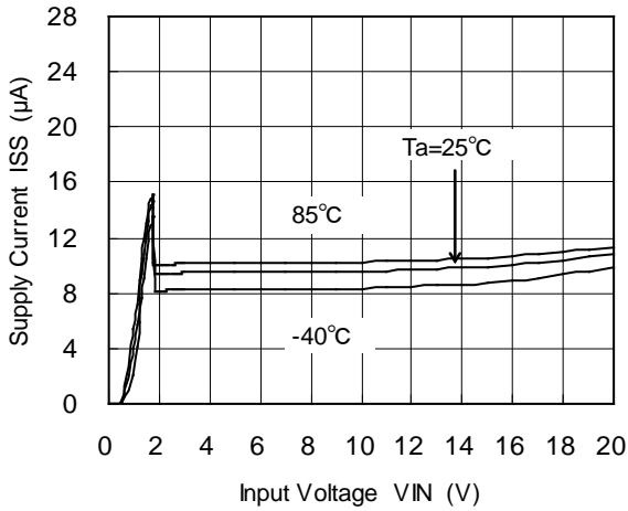
XC6202P182(1.8V)
